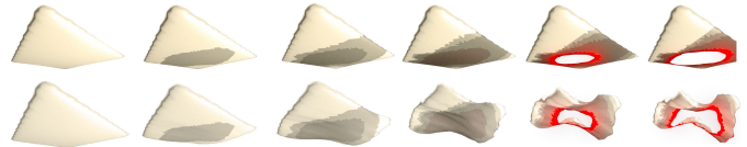
Figure 3: Crumpling paper during burning. (a) decomposition alone, (b) decomposition and crumpling. Flames are not show.
